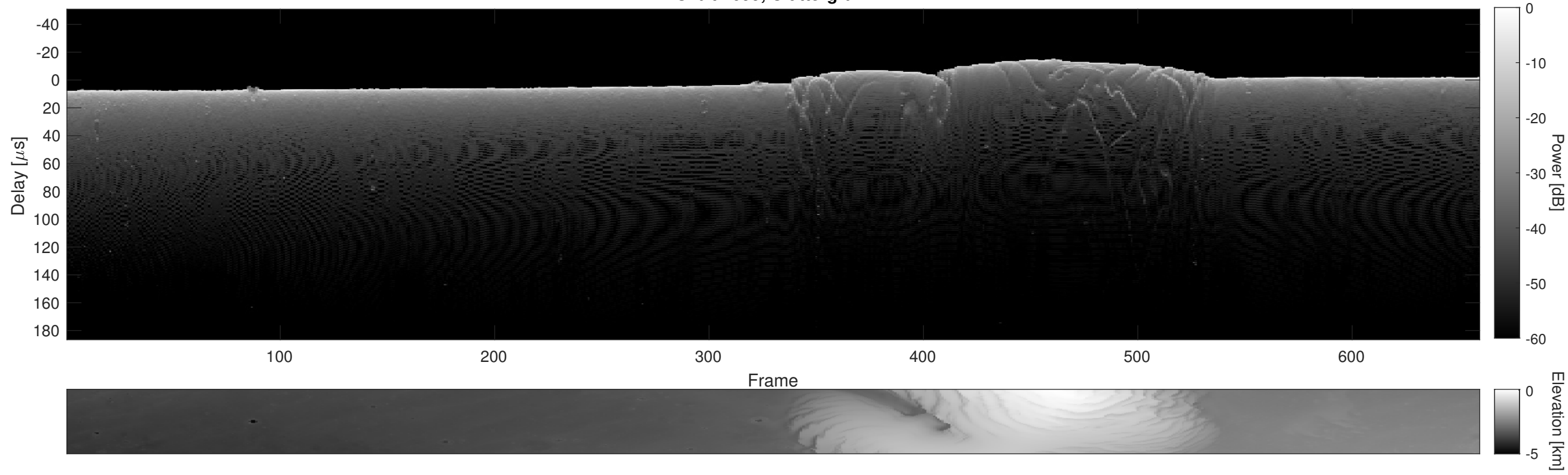
Orbit 7699, Cluttergram
