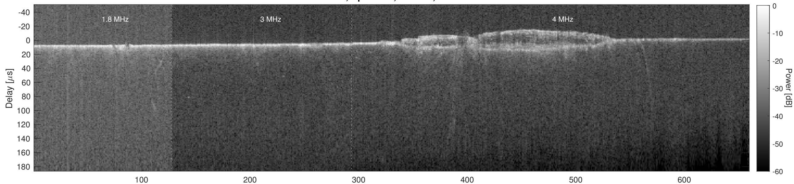
Orbit 7699, Cluttergram
