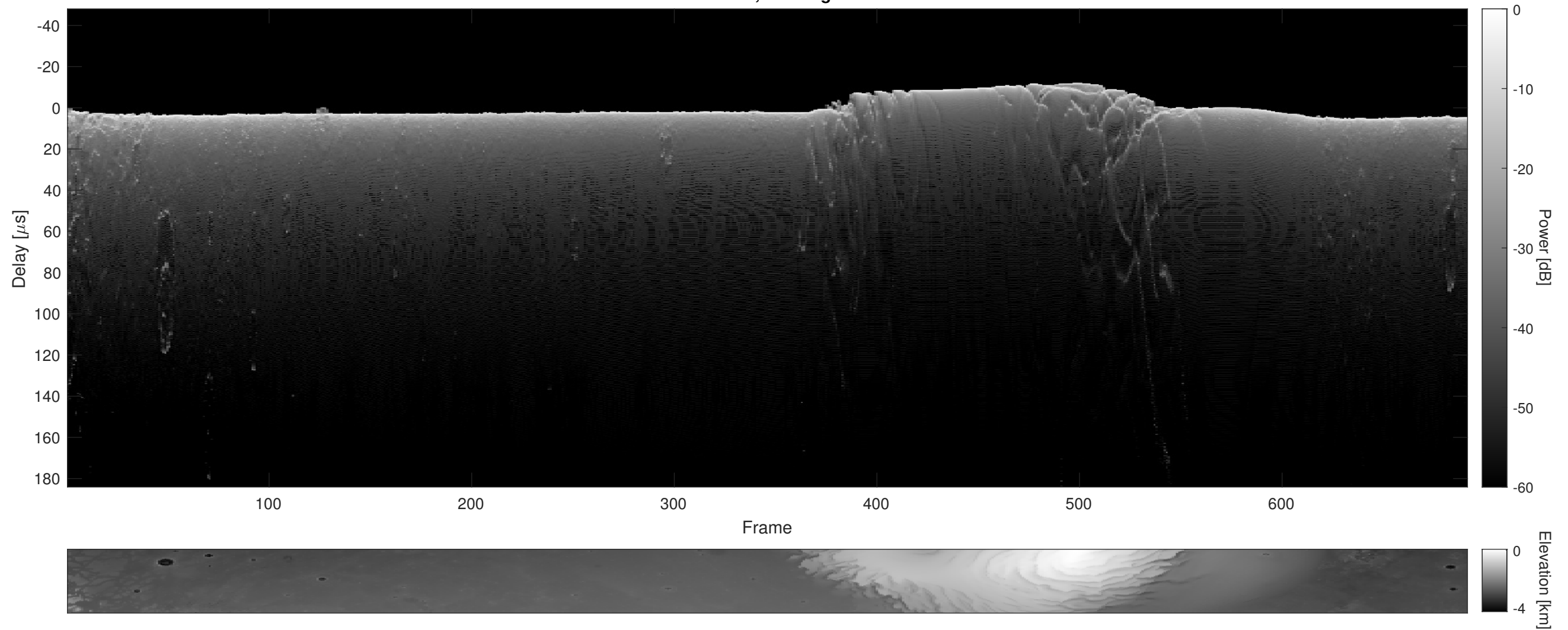
Orbit 7702, Cluttergram
