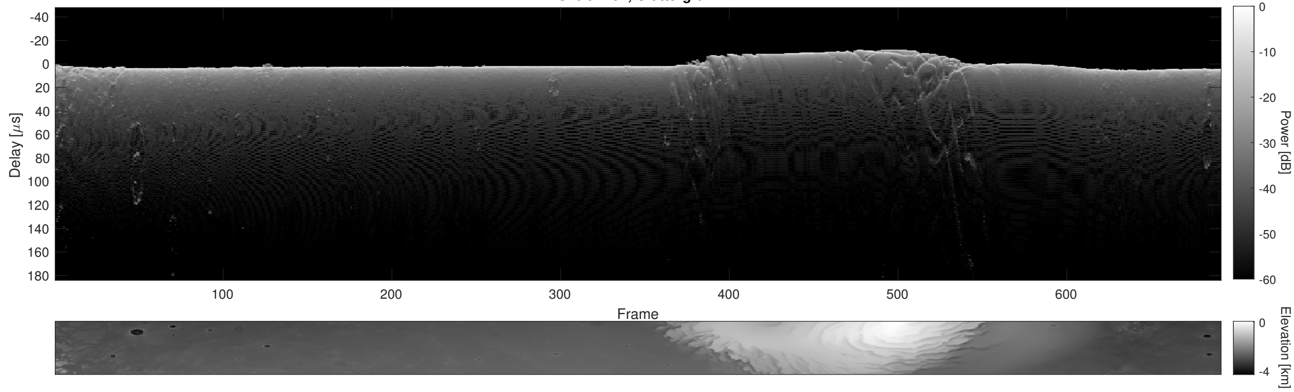
Orbit 7702, Cluttergram
