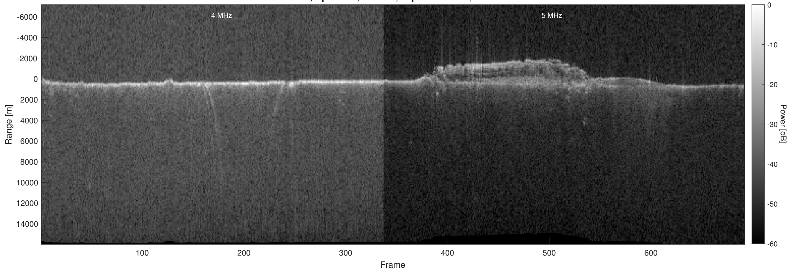
Orbit 7702, Optimized, Window, Depth-Corrected, Channel 2
