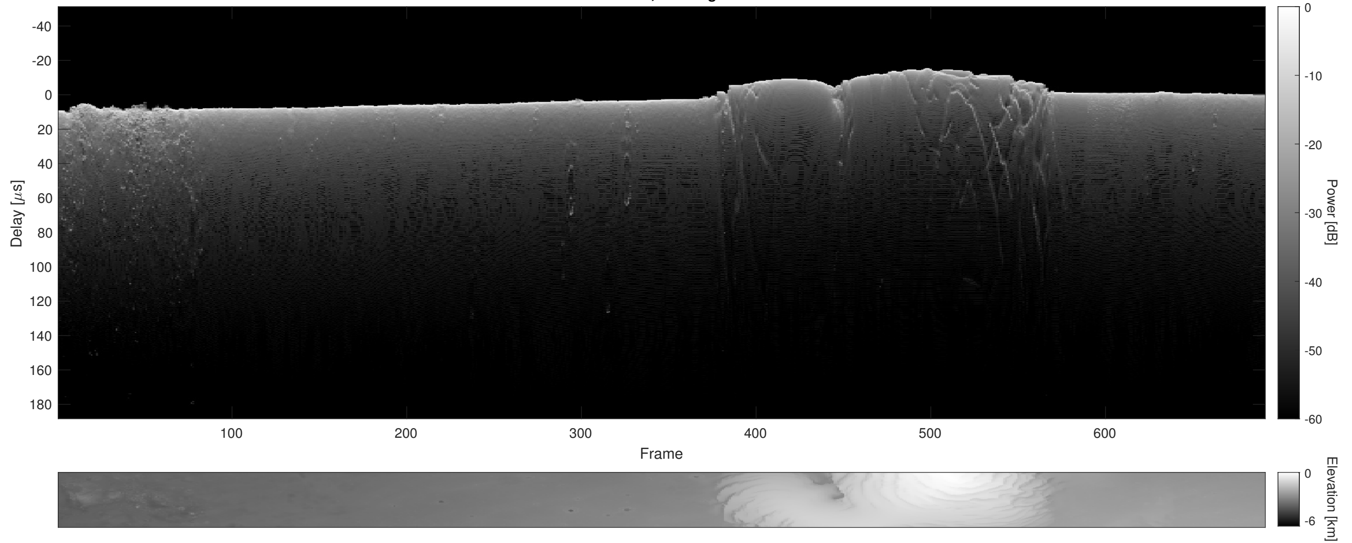
Orbit 7706, Cluttergram
