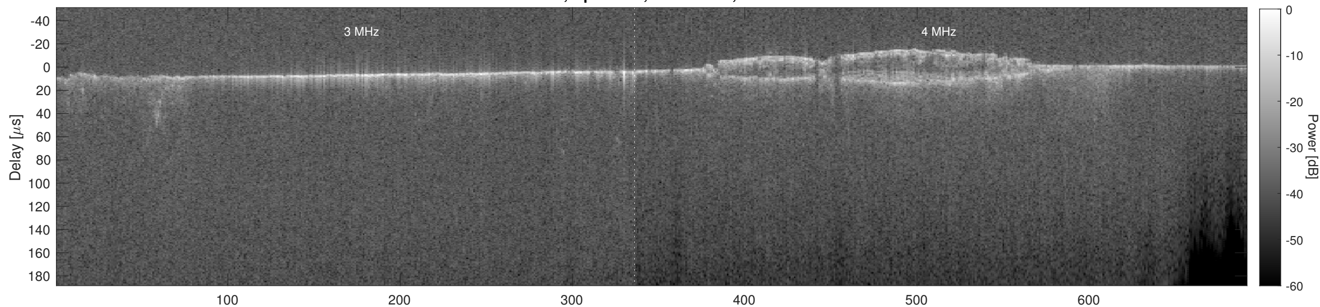
Orbit 7706, Cluttergram
