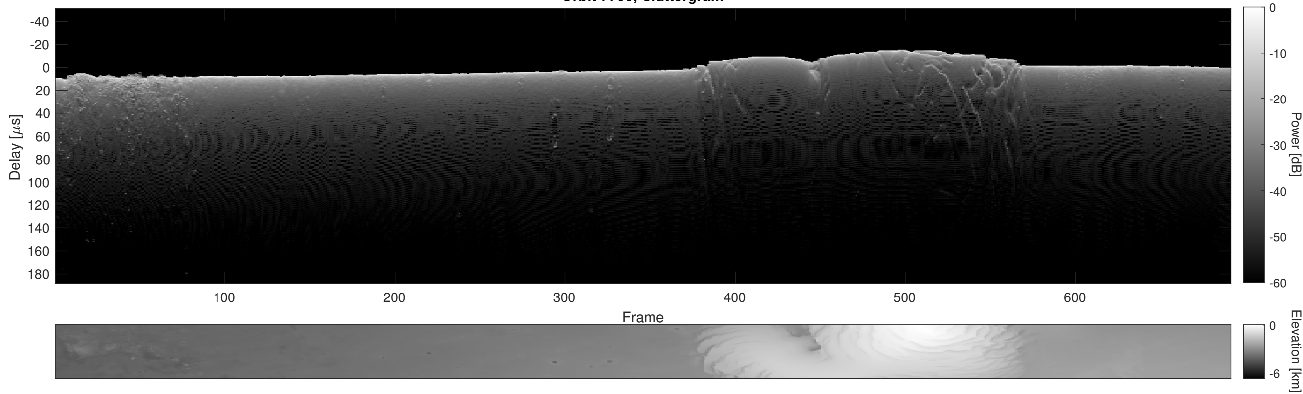
Orbit 7706, Cluttergram
