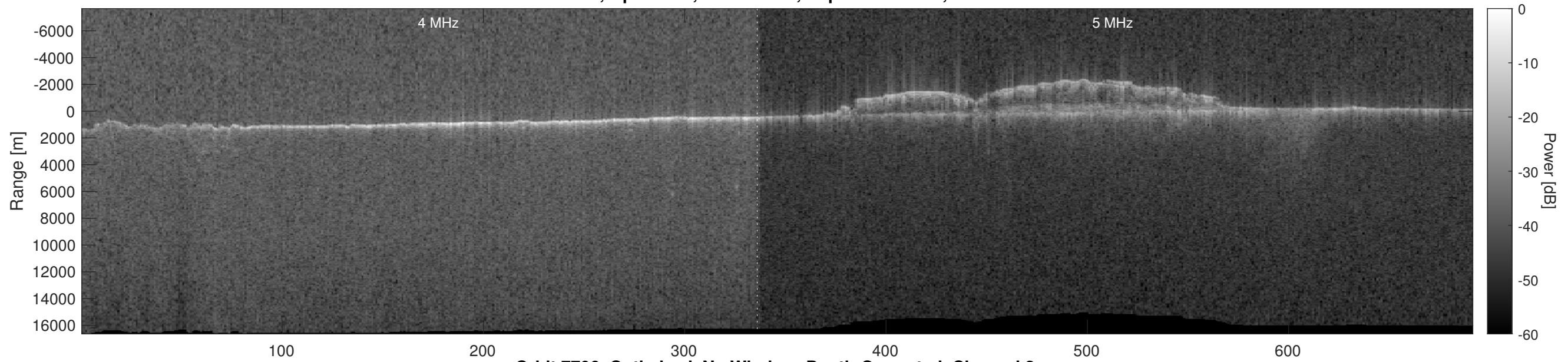
Orbit 7706, Optimized, No Window, Depth-Corrected, Channel 2
