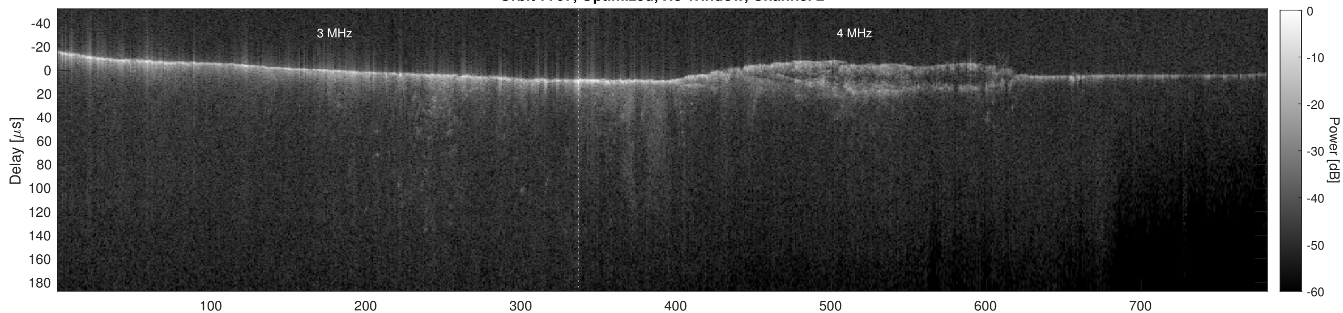
Orbit 7707, Cluttergram
