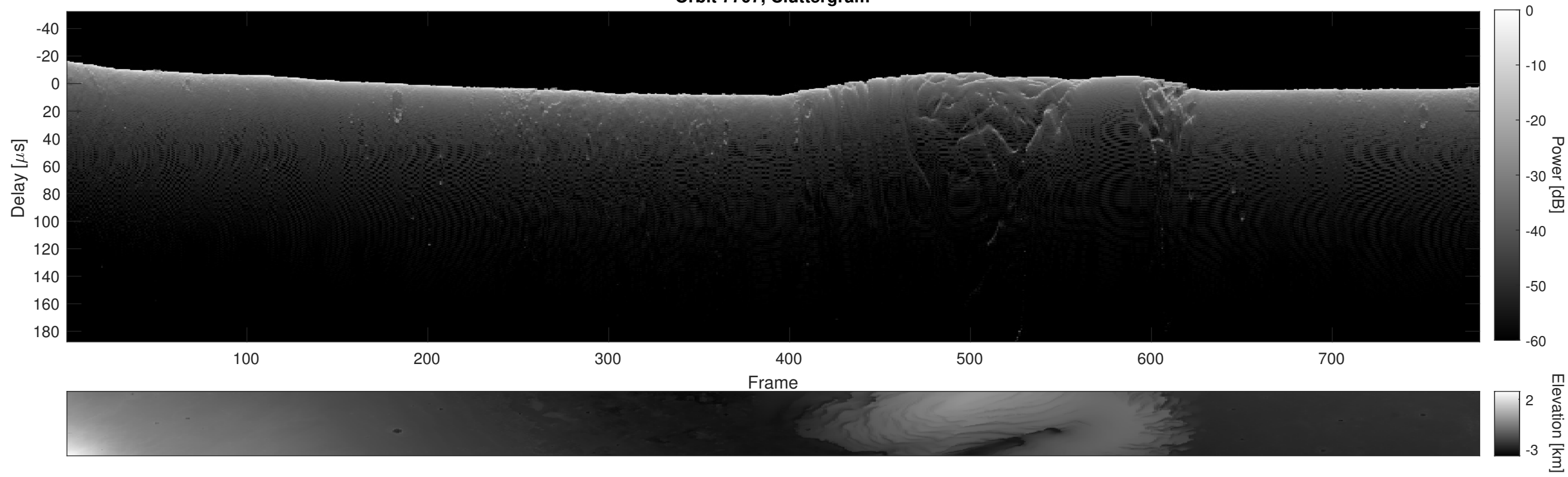
Orbit 7707, Cluttergram
