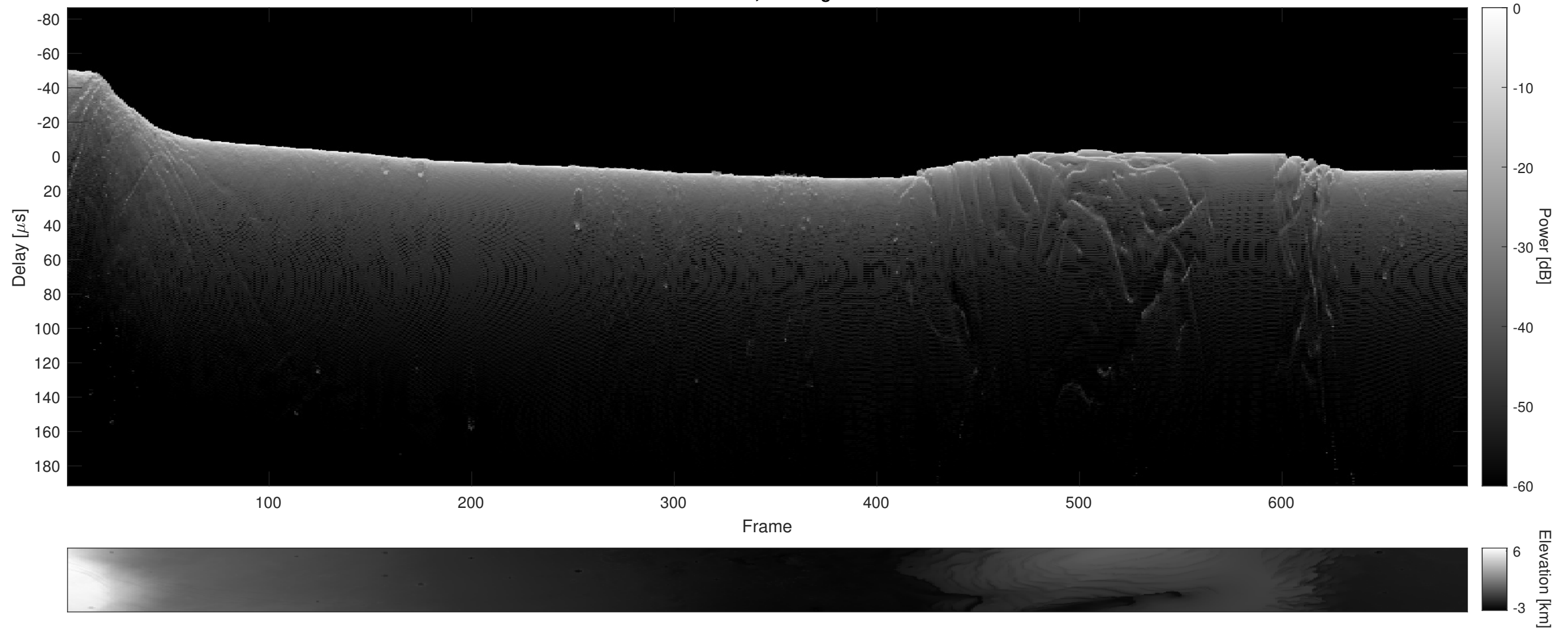
Orbit 7714, Cluttergram
