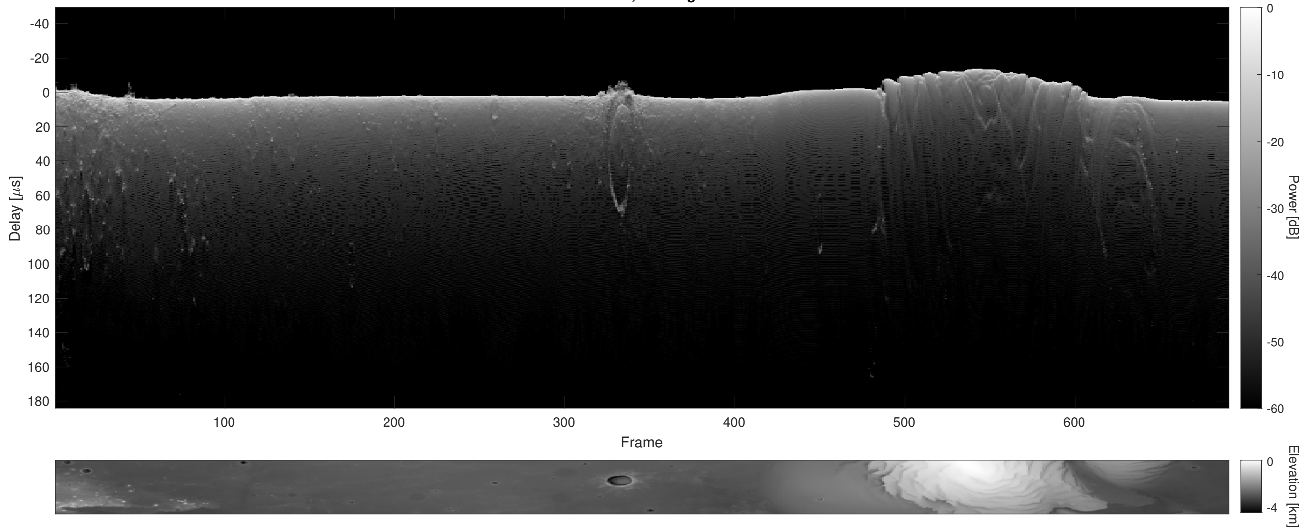
Orbit 7722, Cluttergram
