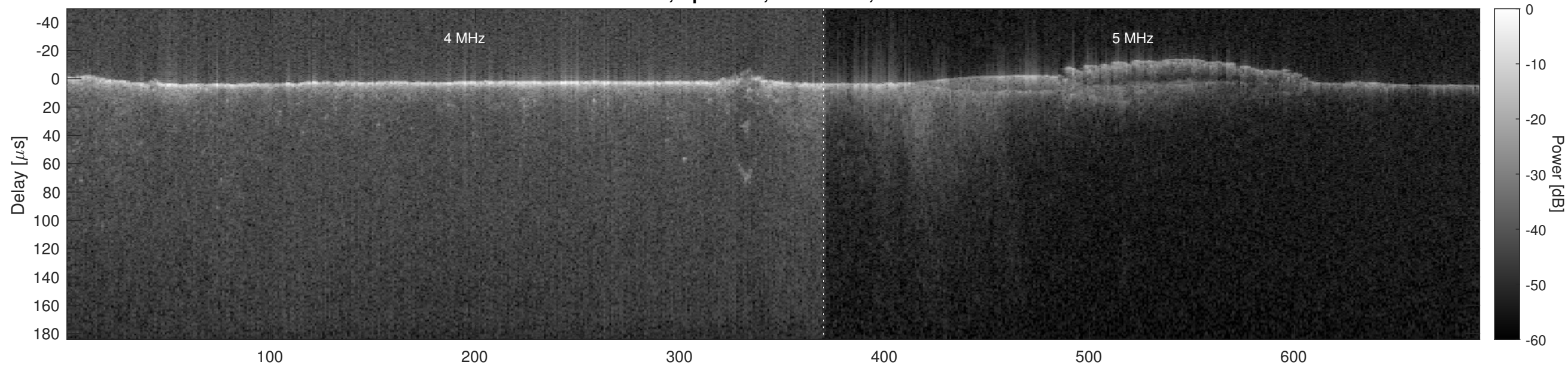
Orbit 7722, Optimized, No Window, Channel 2
