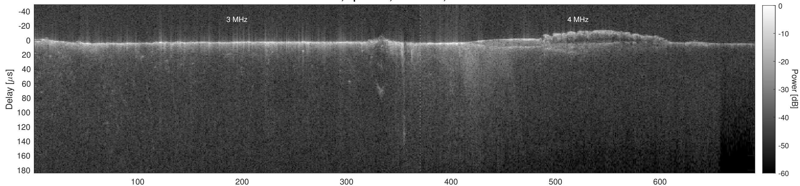
Orbit 7722, Cluttergram
