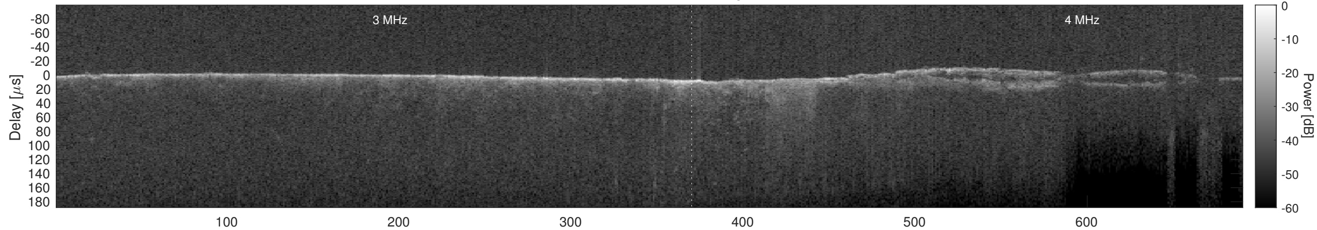
Orbit 7725, Cluttergram
