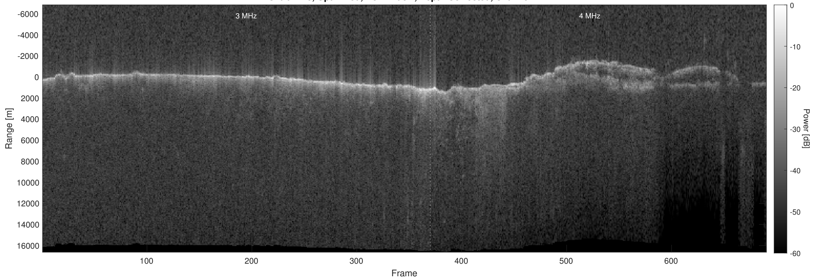
Orbit 7725, Optimized, No Window, Depth-Corrected, Channel 2
