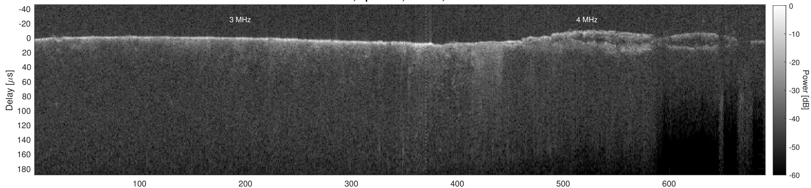
Orbit 7725, Cluttergram
