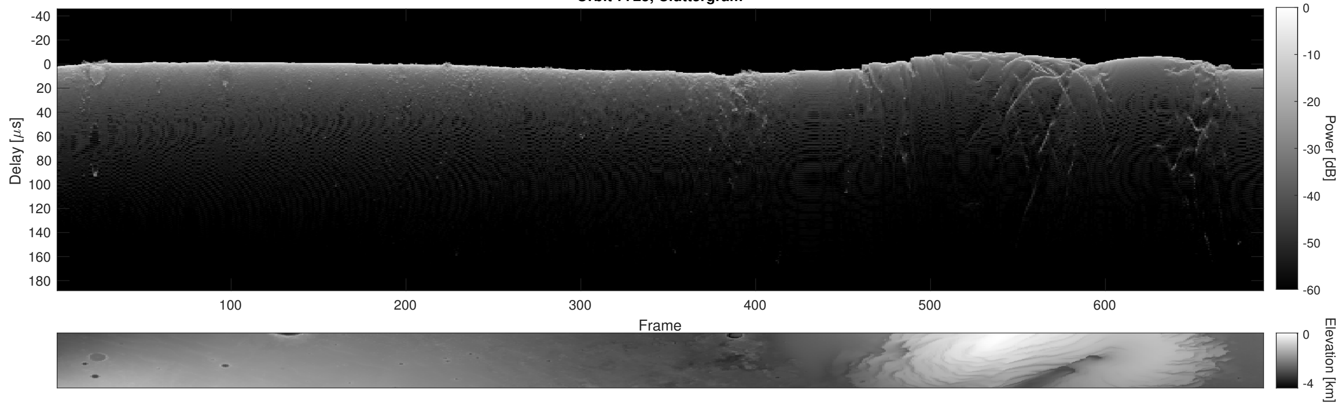
Orbit 7725, Cluttergram
