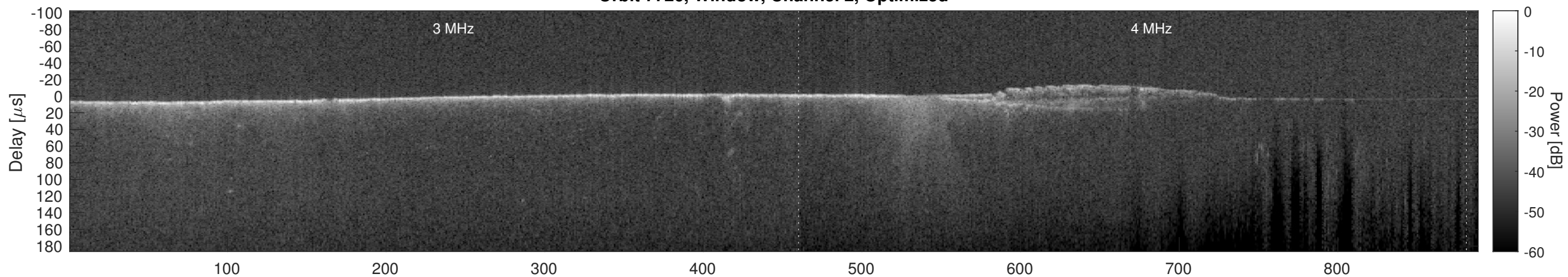
Orbit 7726, Cluttergram
