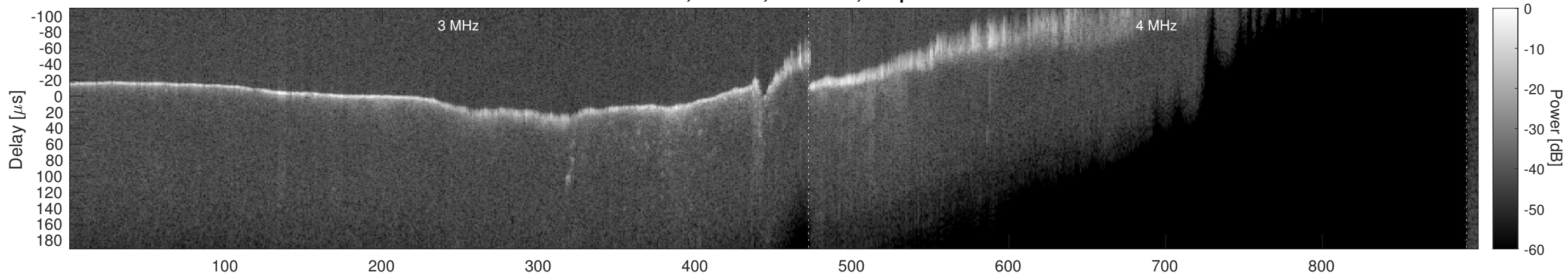
Orbit 7732, Window, Channel 2, Optimized
