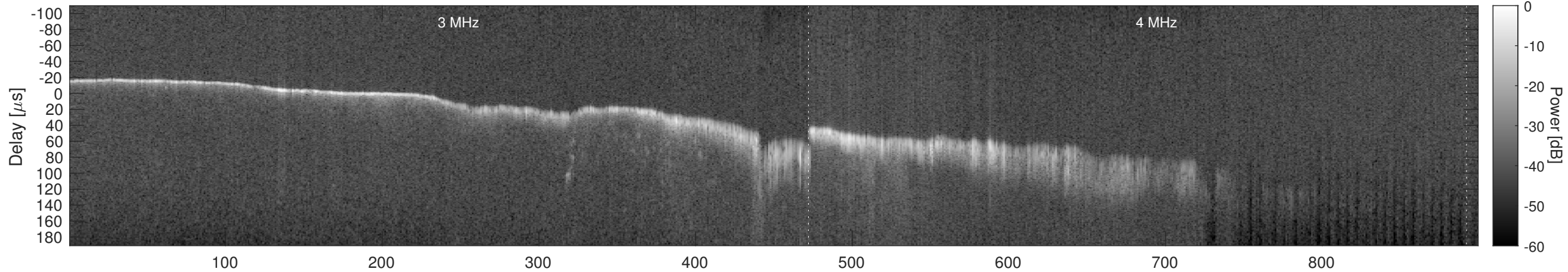
Orbit 7732, Window, Channel 2, Chapman
