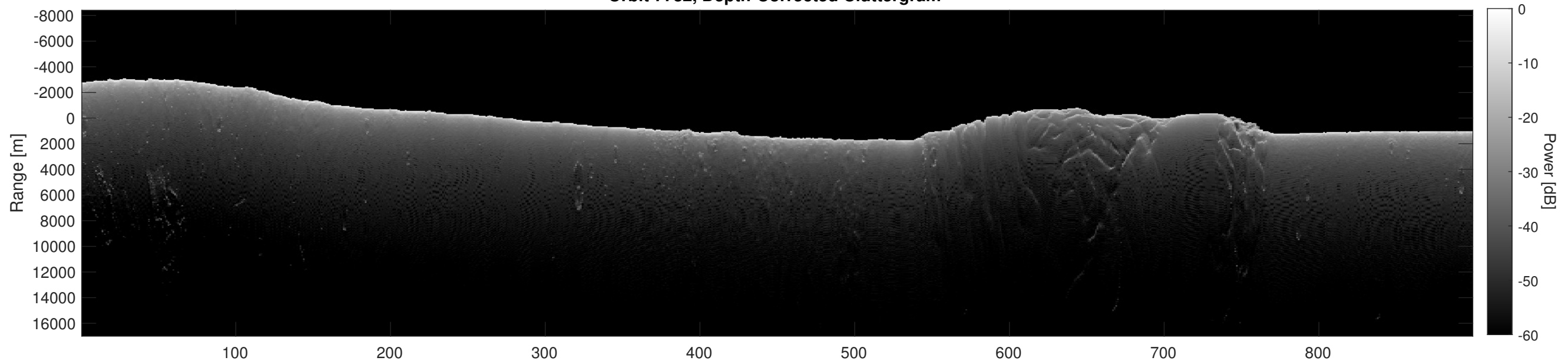
Orbit 7732, Depth-Corrected Cluttergram
