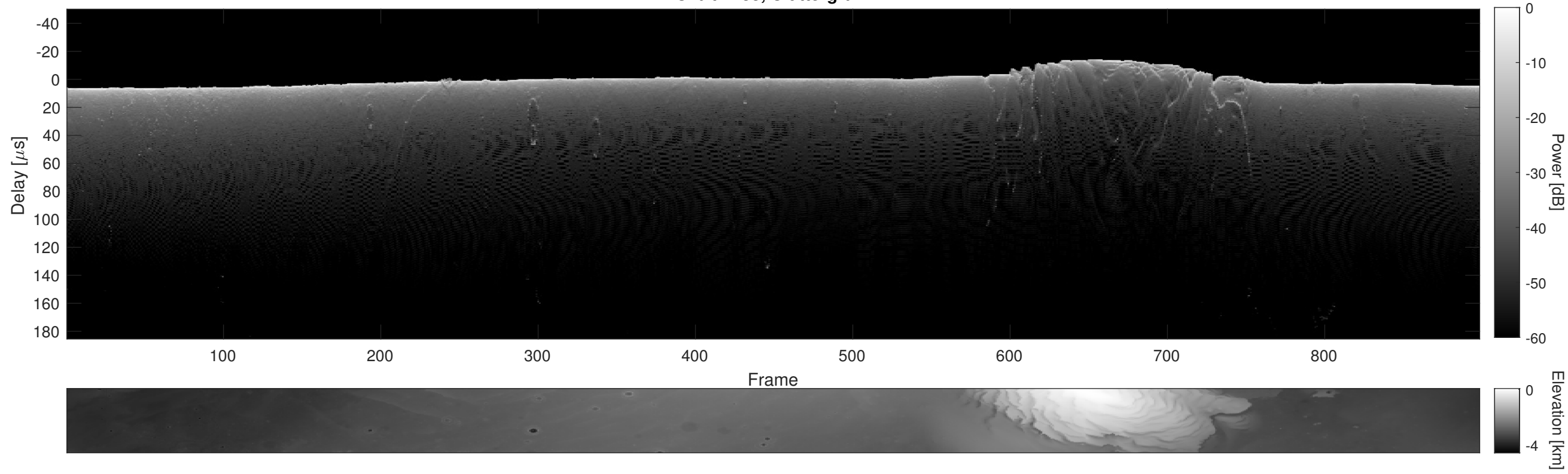
Orbit 7733, Cluttergram
