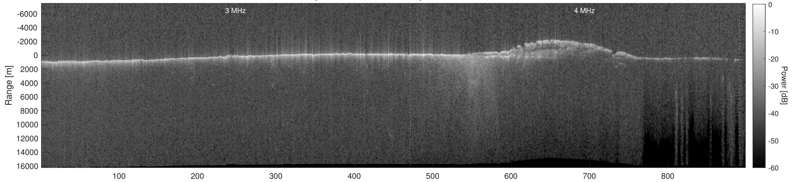
Orbit 7733, Depth-Corrected Cluttergram
