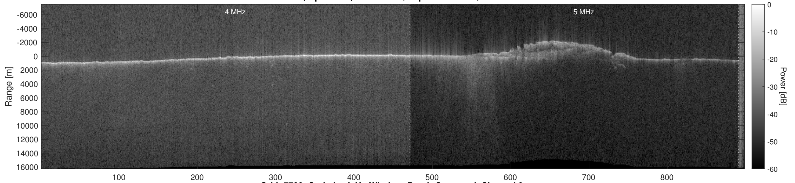
Orbit 7733, Optimized, No Window, Depth-Corrected, Channel 2
