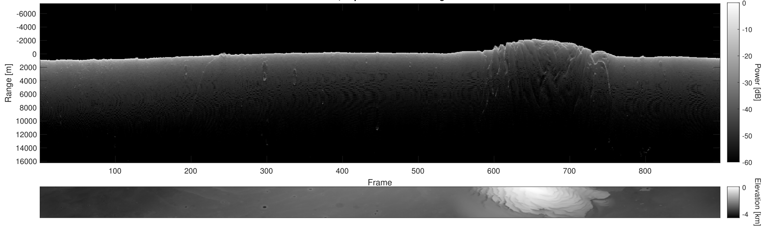
Orbit 7733, Depth-Corrected Cluttergram
