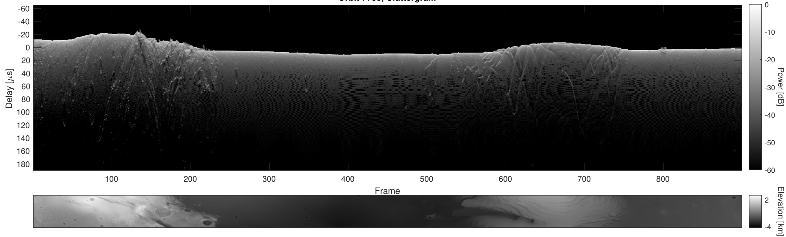
Orbit 7735, Cluttergram
