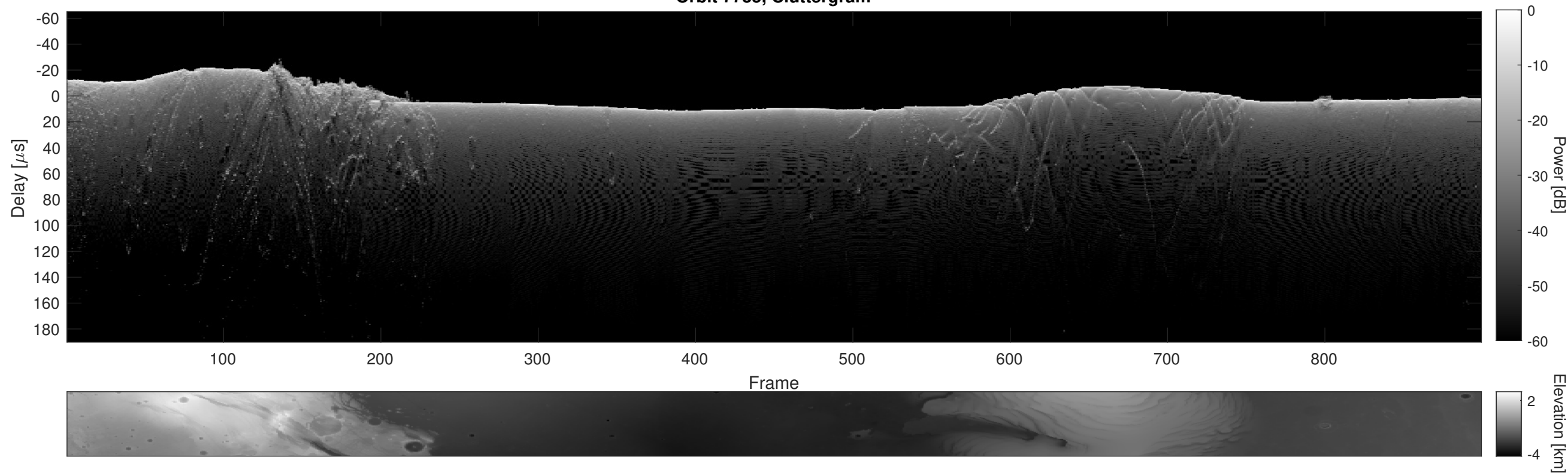
Orbit 7735, Cluttergram
