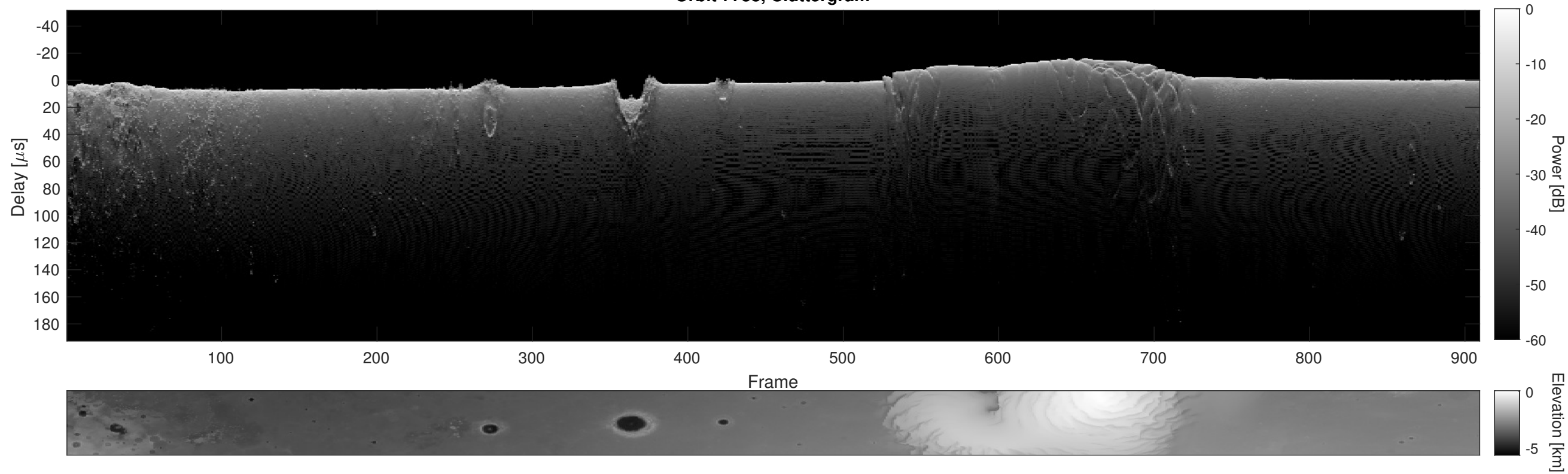
Orbit 7738, Cluttergram
