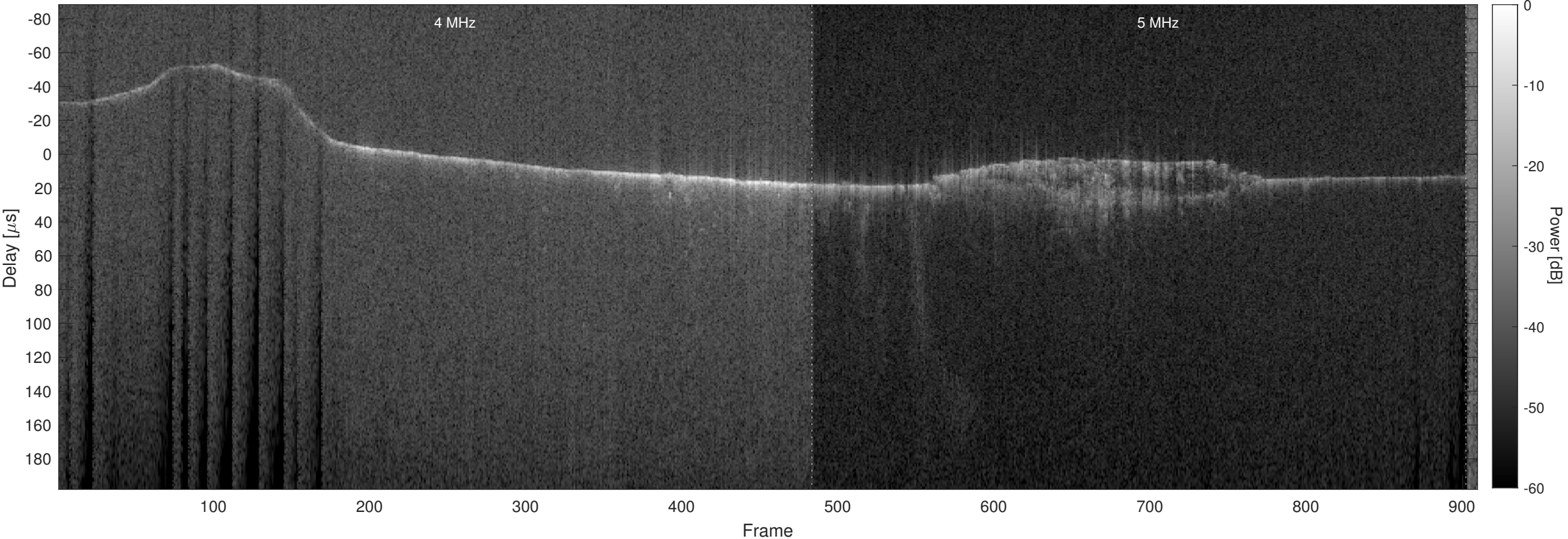
Orbit 7739, Optimized, No Window, Channel 2
