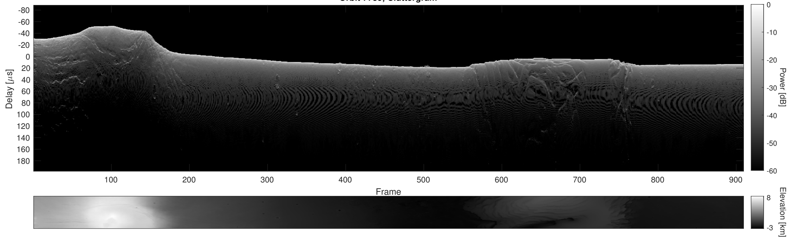
Orbit 7739, Cluttergram
