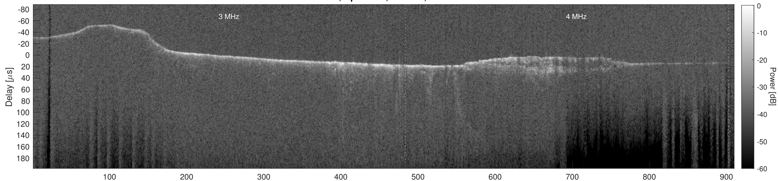
Orbit 7739, Cluttergram
