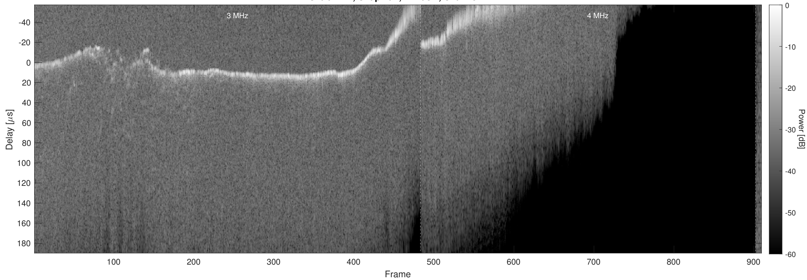
Orbit 7741, Chapman, Window, Channel 2
