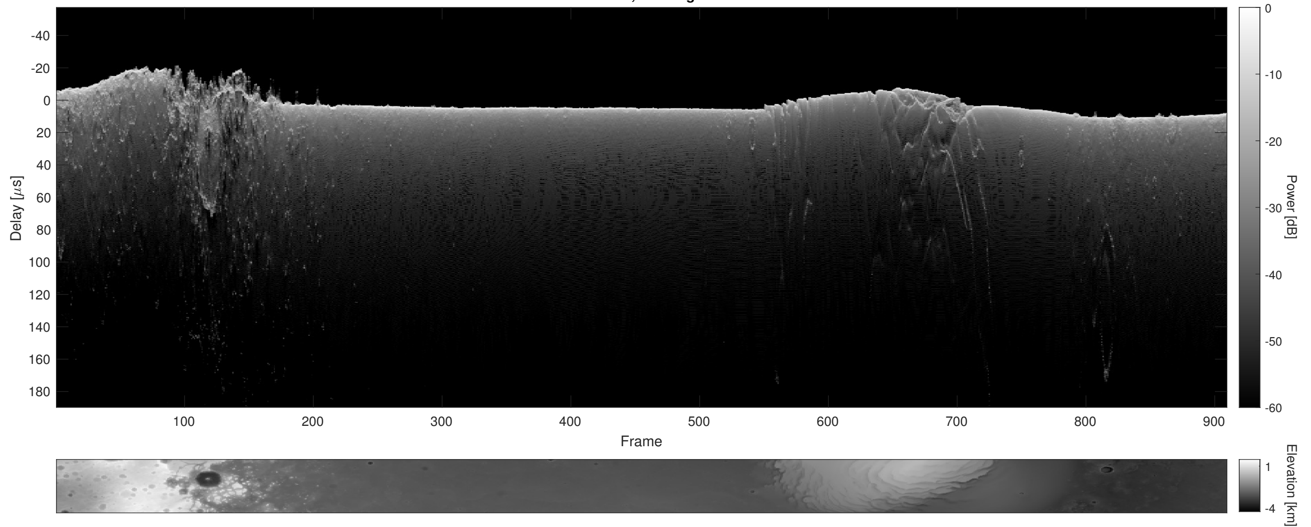
Orbit 7741, Cluttergram
