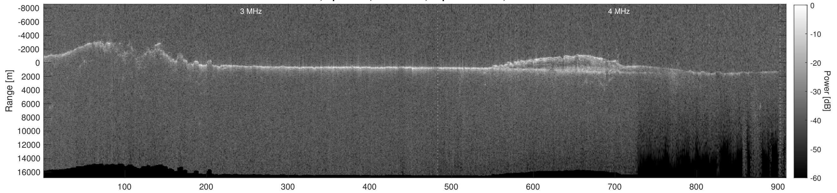
Orbit 7741, Depth-Corrected Cluttergram
