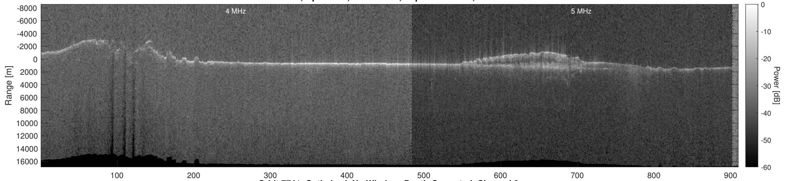
Orbit 7741, Optimized, No Window, Depth-Corrected, Channel 2
