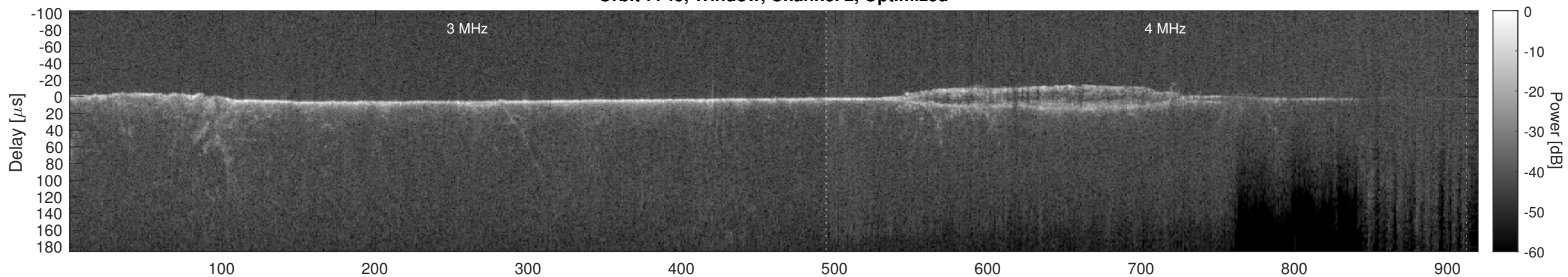
Orbit 7745, Cluttergram
