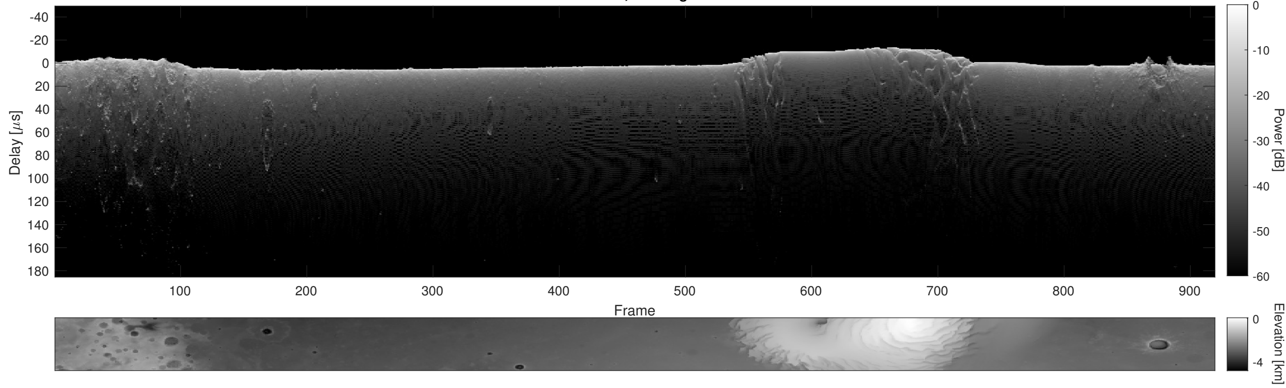
Orbit 7745, Cluttergram
