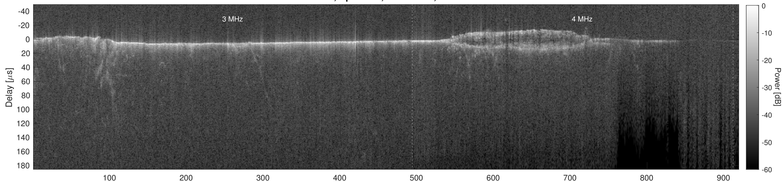
Orbit 7745, Cluttergram
