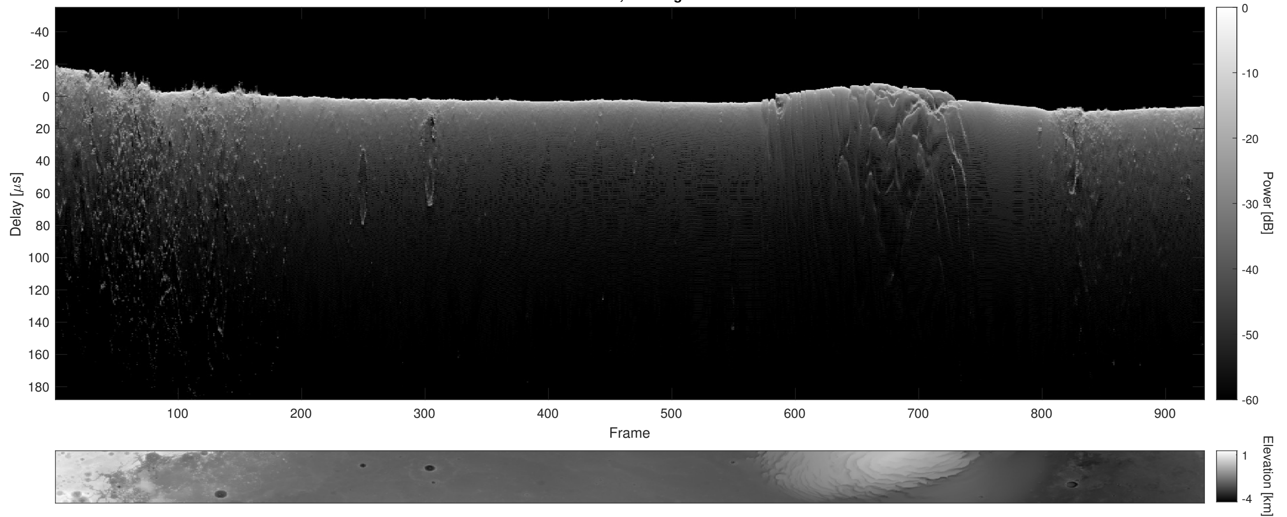
Orbit 7748, Cluttergram
