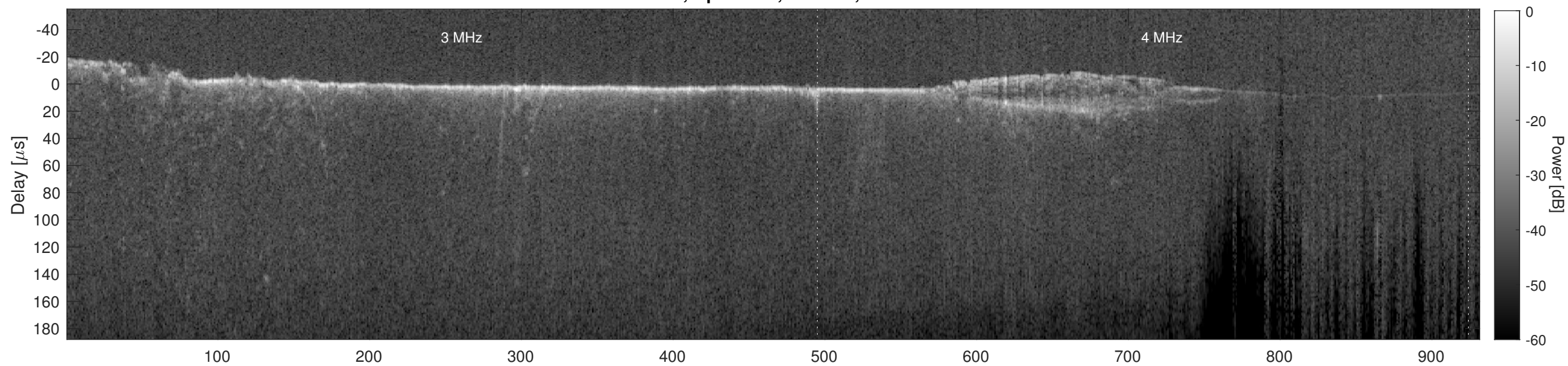
Orbit 7748, Cluttergram
