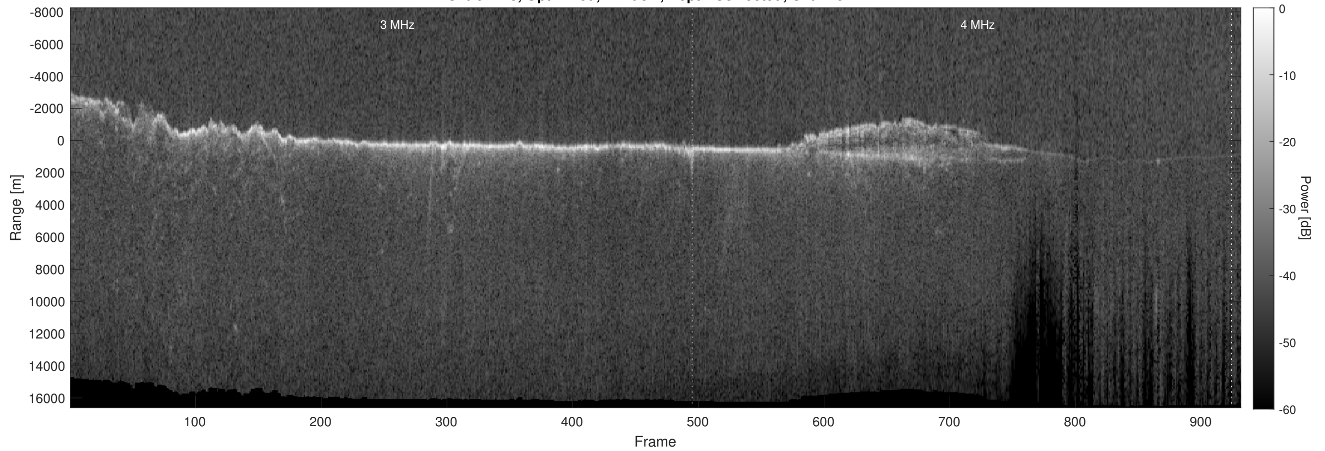
Orbit 7748, Optimized, Window, Depth-Corrected, Channel 2
