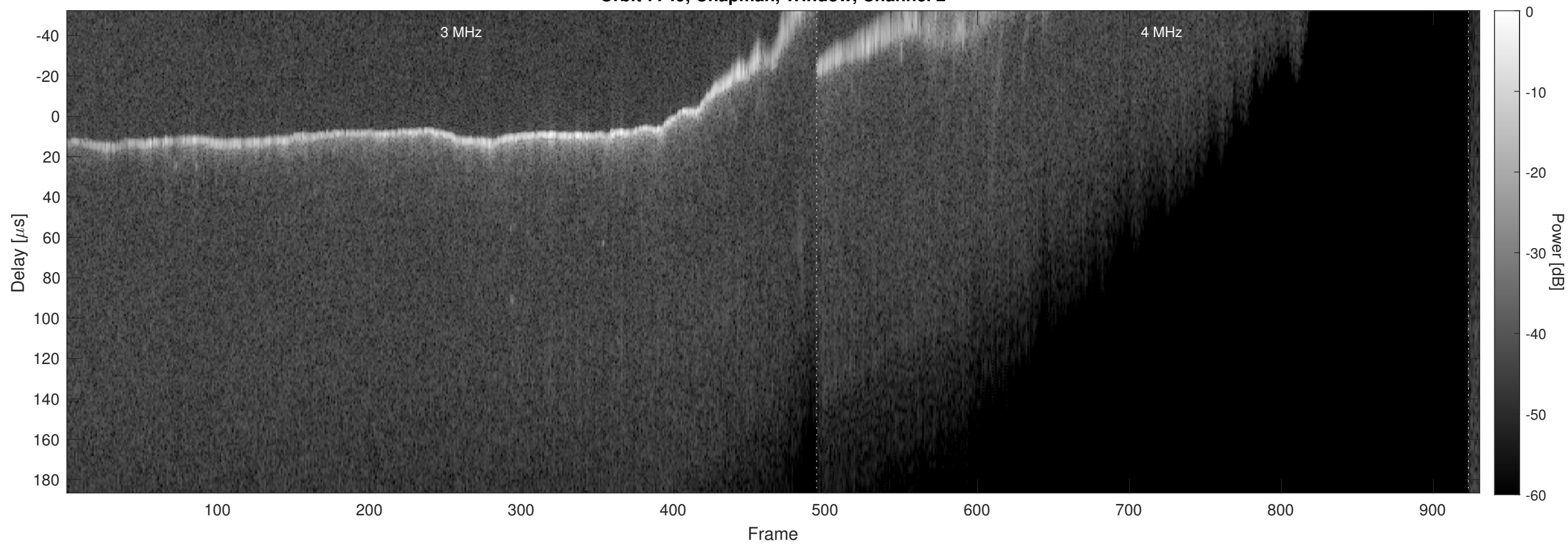
Orbit 7749, Chapman, Window, Channel 2
