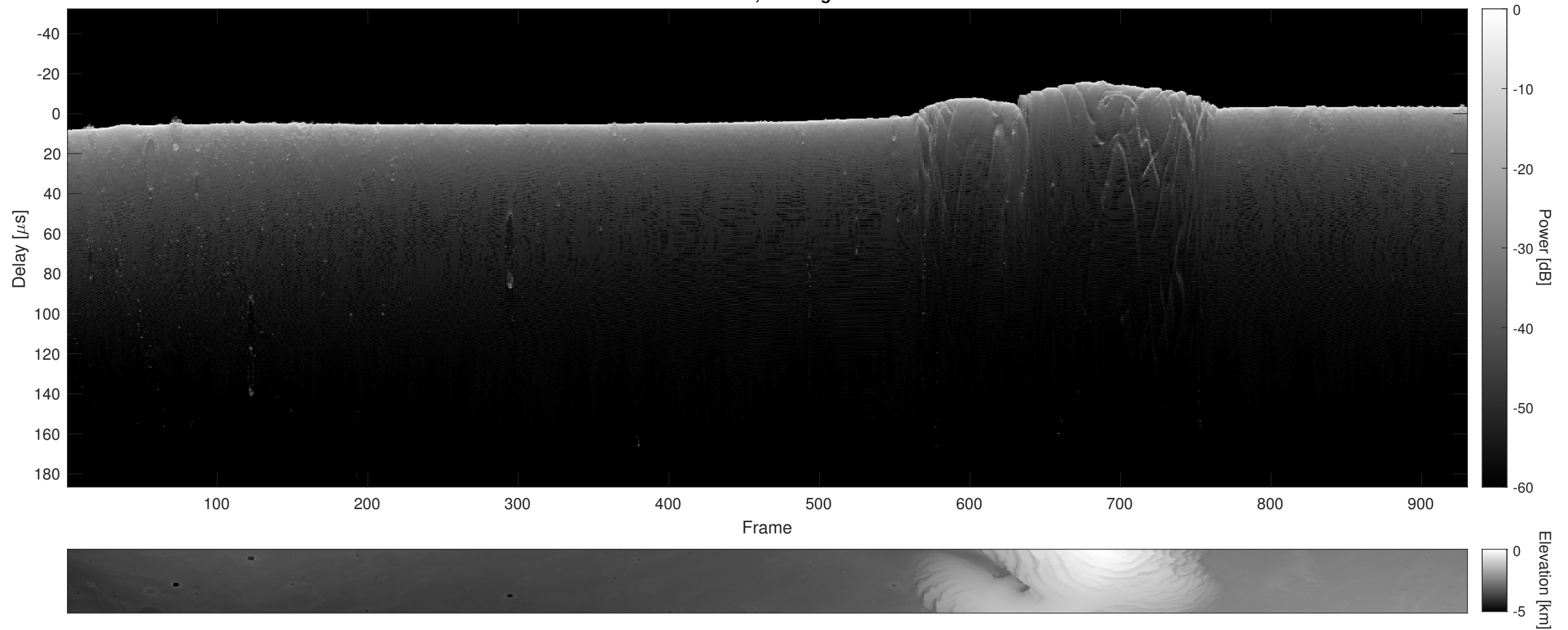
Orbit 7749, Cluttergram
