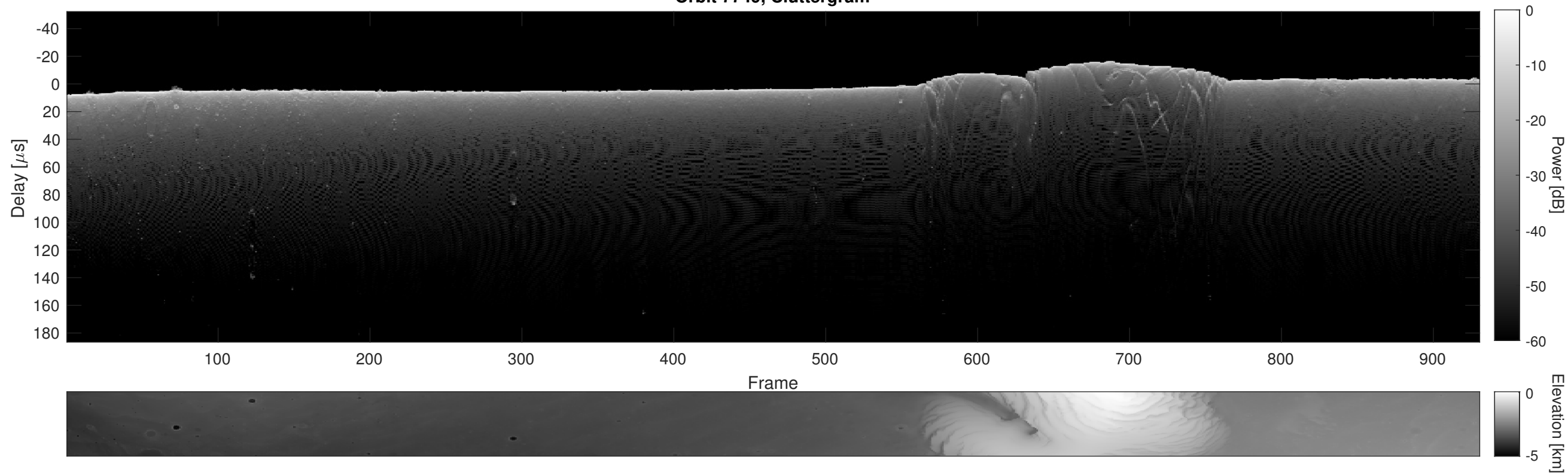
Orbit 7749, Cluttergram
