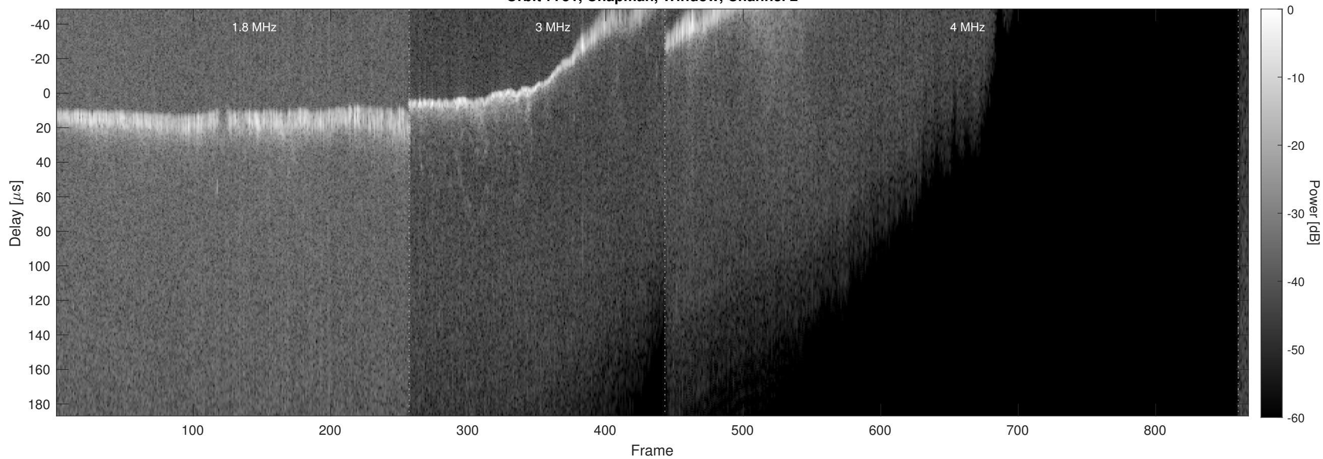
Orbit 7751, Chapman, Window, Channel 2
