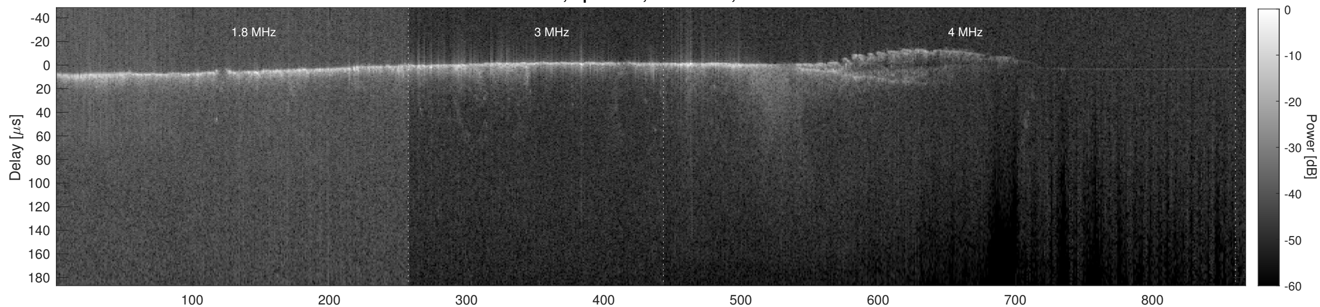
Orbit 7751, Cluttergram
