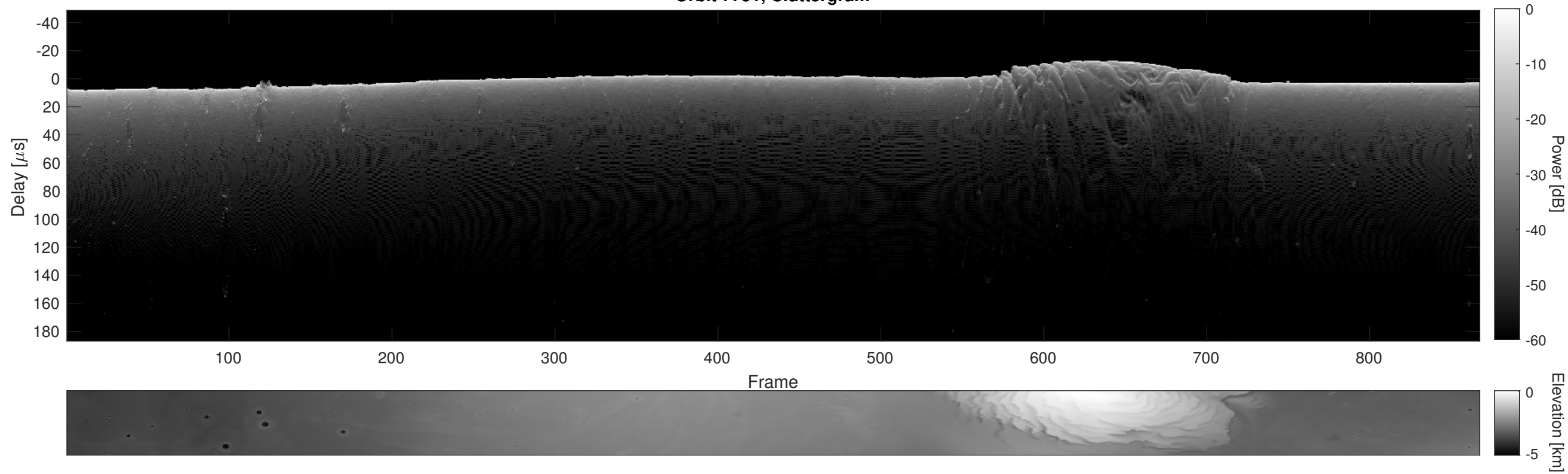
Orbit 7751, Cluttergram
