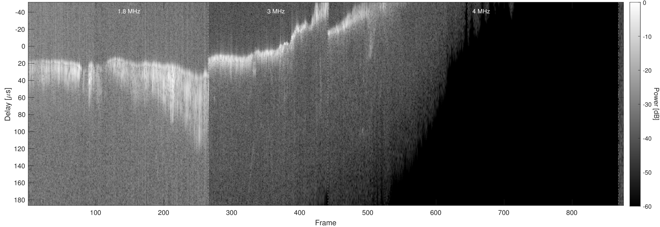
Orbit 7754, Chapman, No Window, Channel 2
