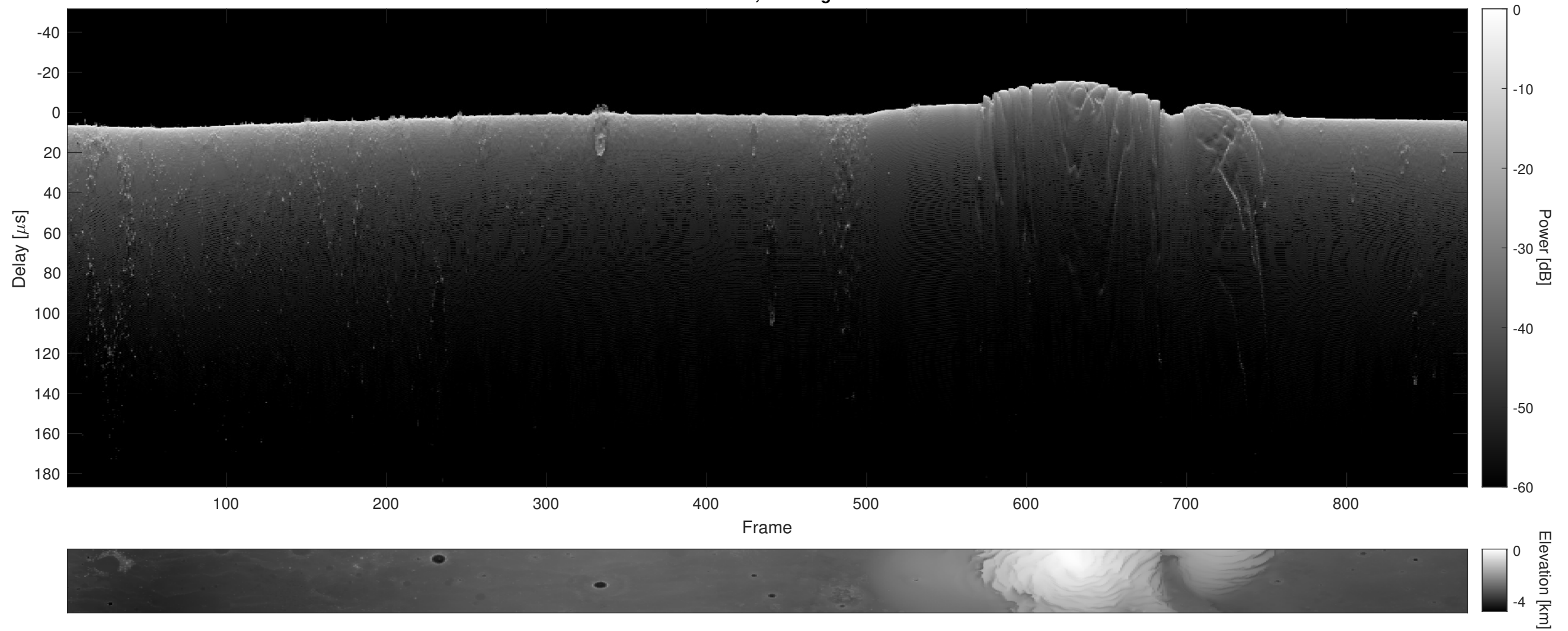
Orbit 7754, Cluttergram
