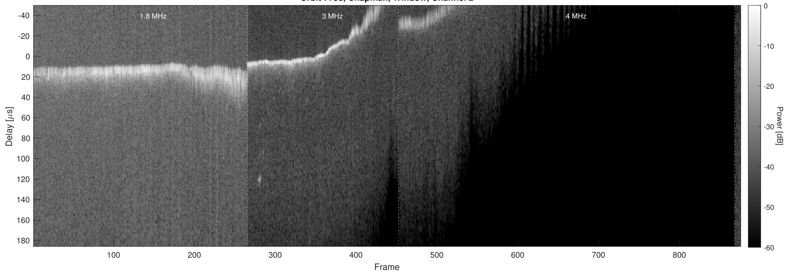
Orbit 7758, Chapman, Window, Channel 2
