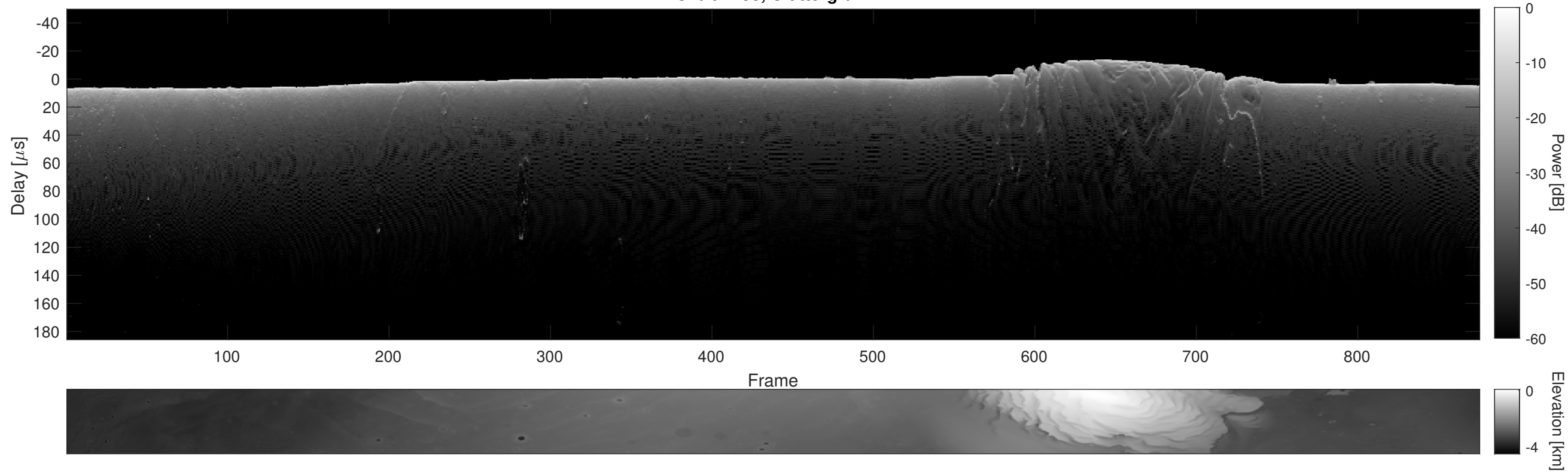
Orbit 7758, Cluttergram
