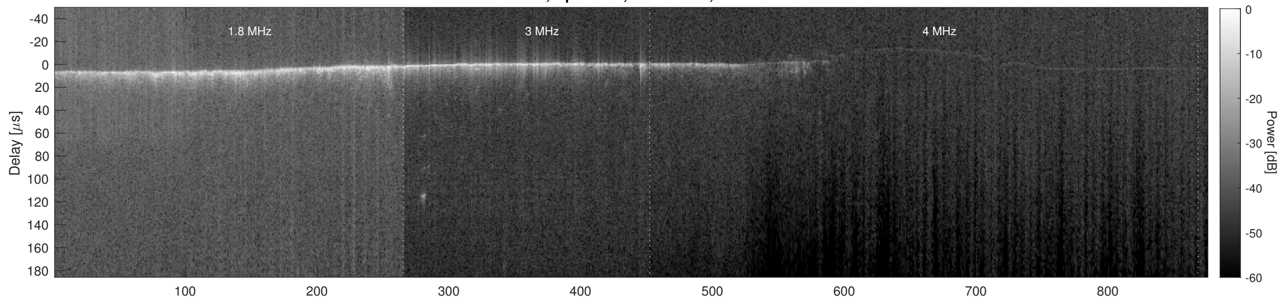
Orbit 7758, Cluttergram
