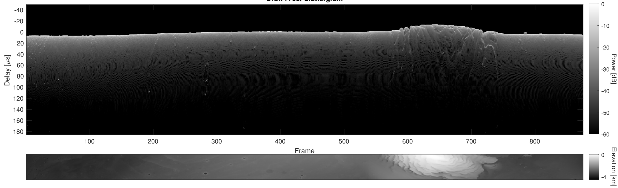
Orbit 7758, Cluttergram
