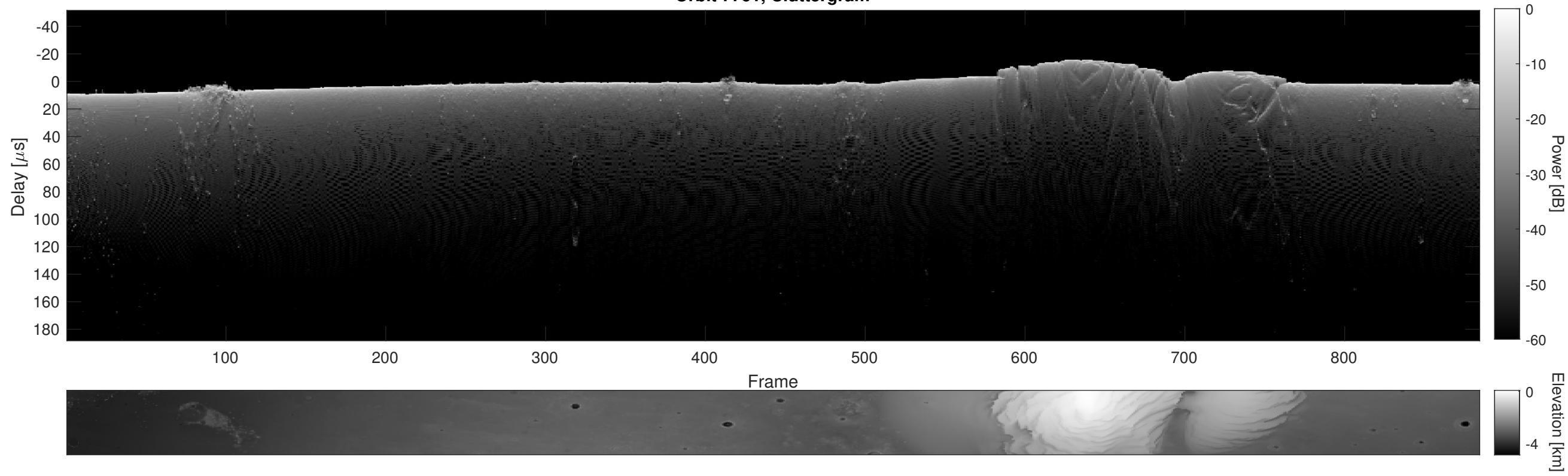
Orbit 7761, Cluttergram
