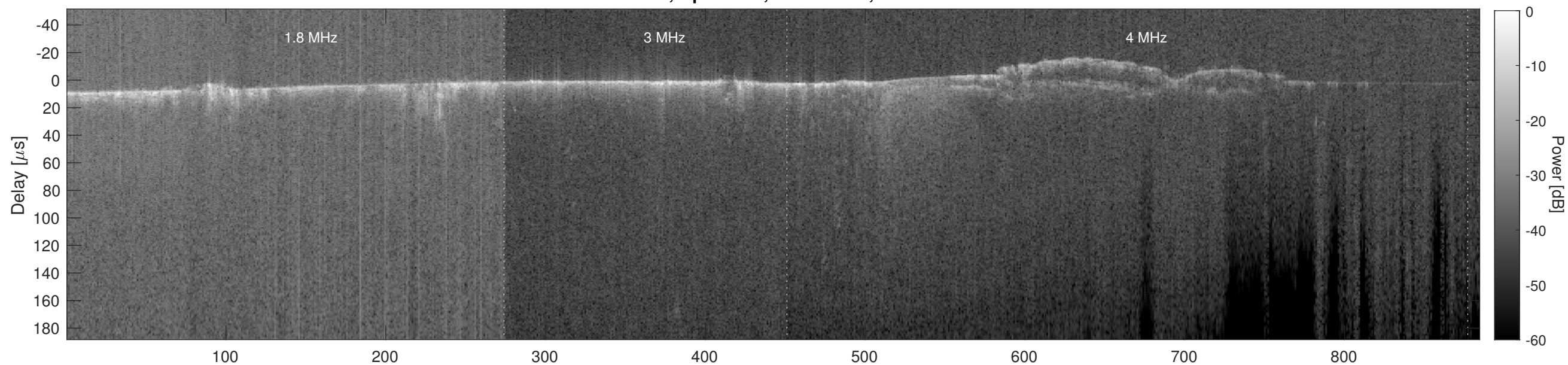
Orbit 7761, Cluttergram
