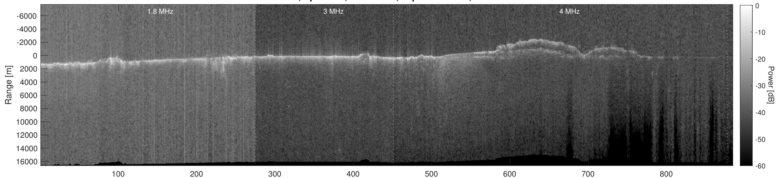
Orbit 7761, Depth-Corrected Cluttergram
