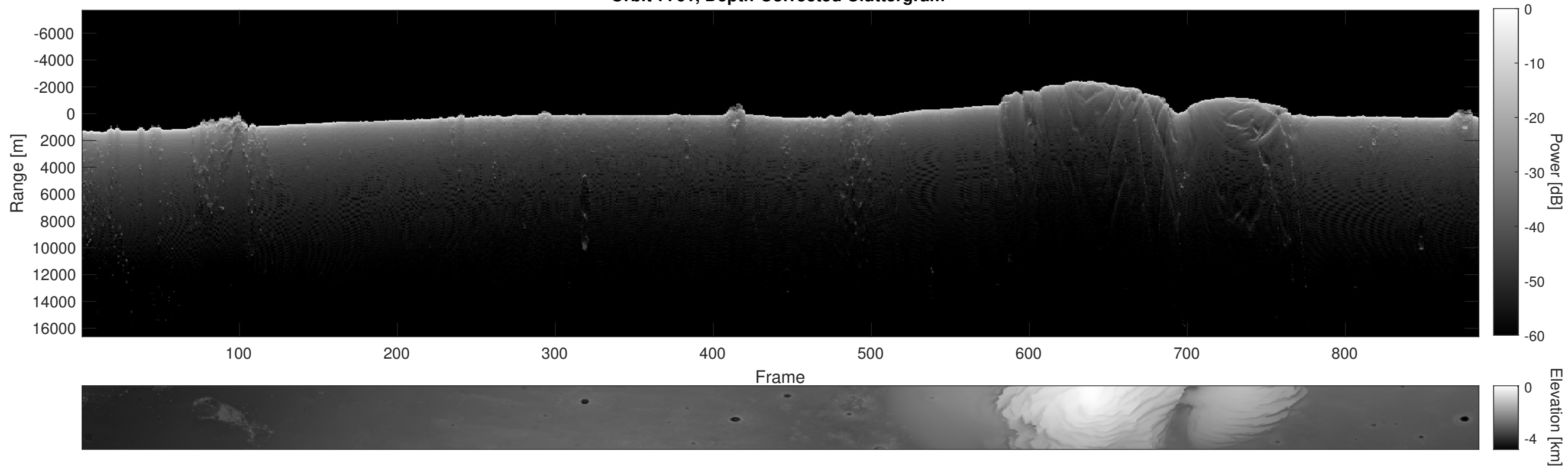
Orbit 7761, Depth-Corrected Cluttergram
