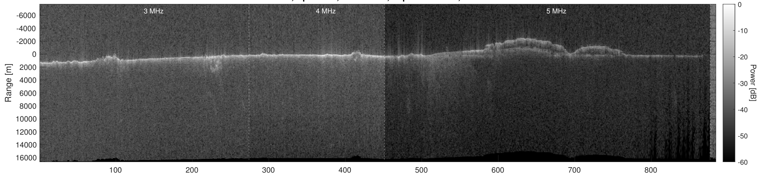
Orbit 7761, Optimized, No Window, Depth-Corrected, Channel 2
