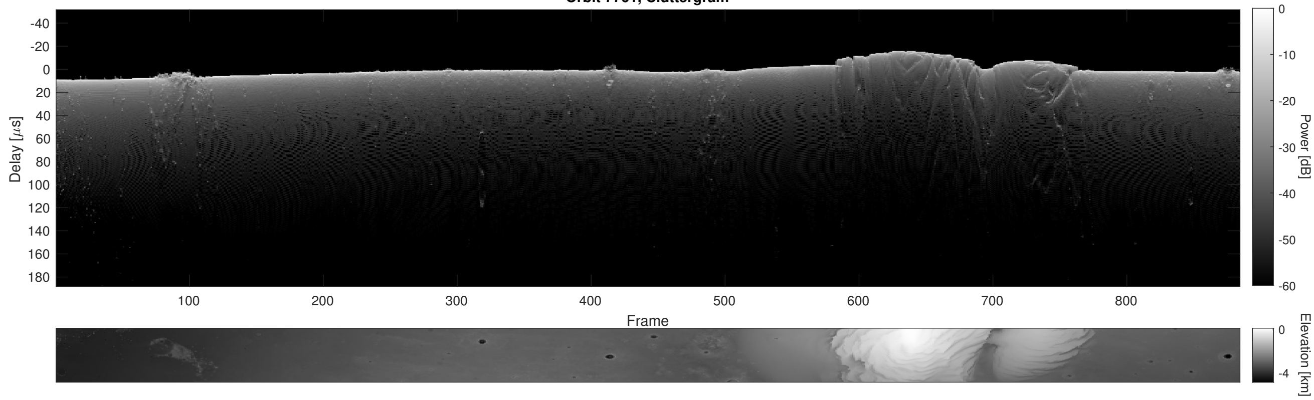
Orbit 7761, Cluttergram
