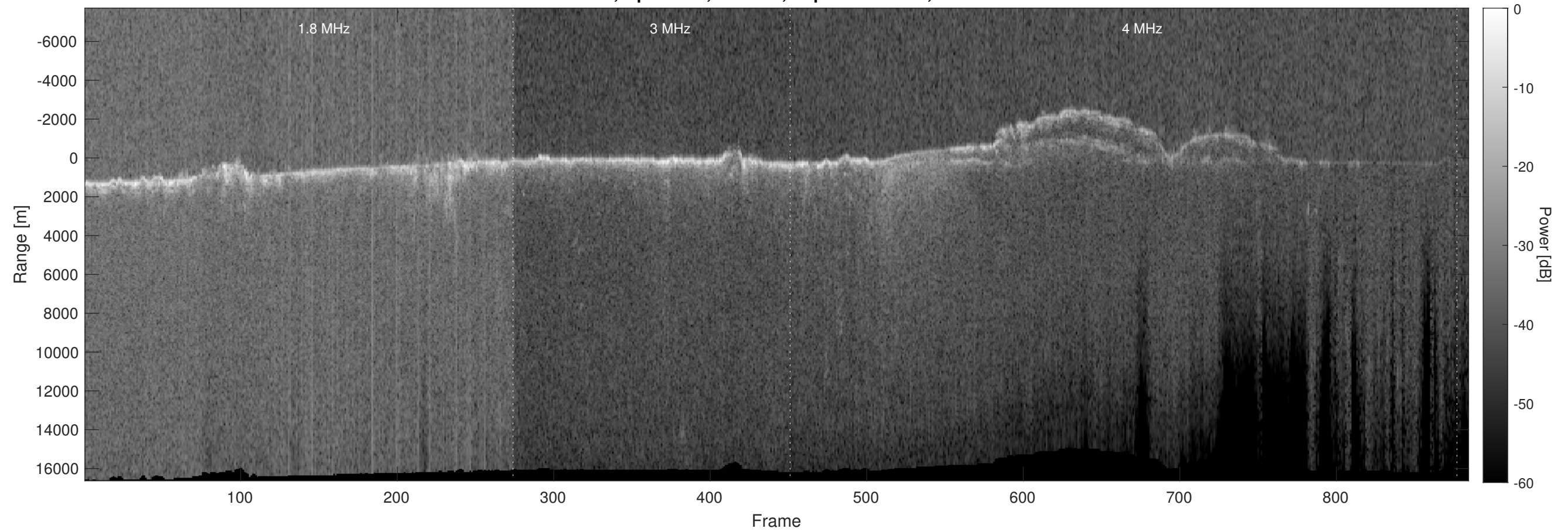
Orbit 7761, Optimized, Window, Depth-Corrected, Channel 2
