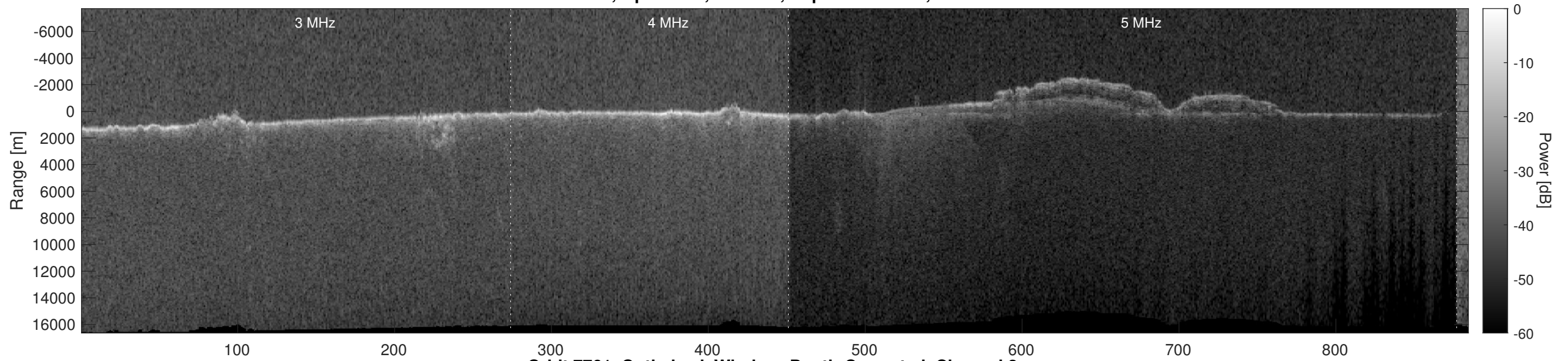
Orbit 7761, Optimized, Window, Depth-Corrected, Channel 2
