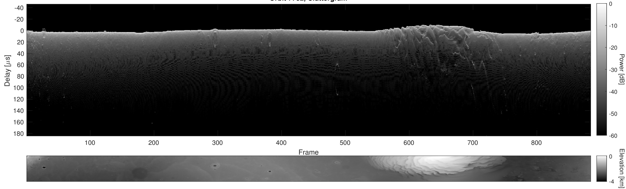
Orbit 7762, Cluttergram
